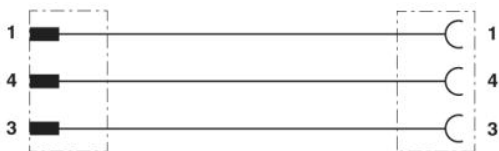
Contact assignment of M8 plugs/sockets
